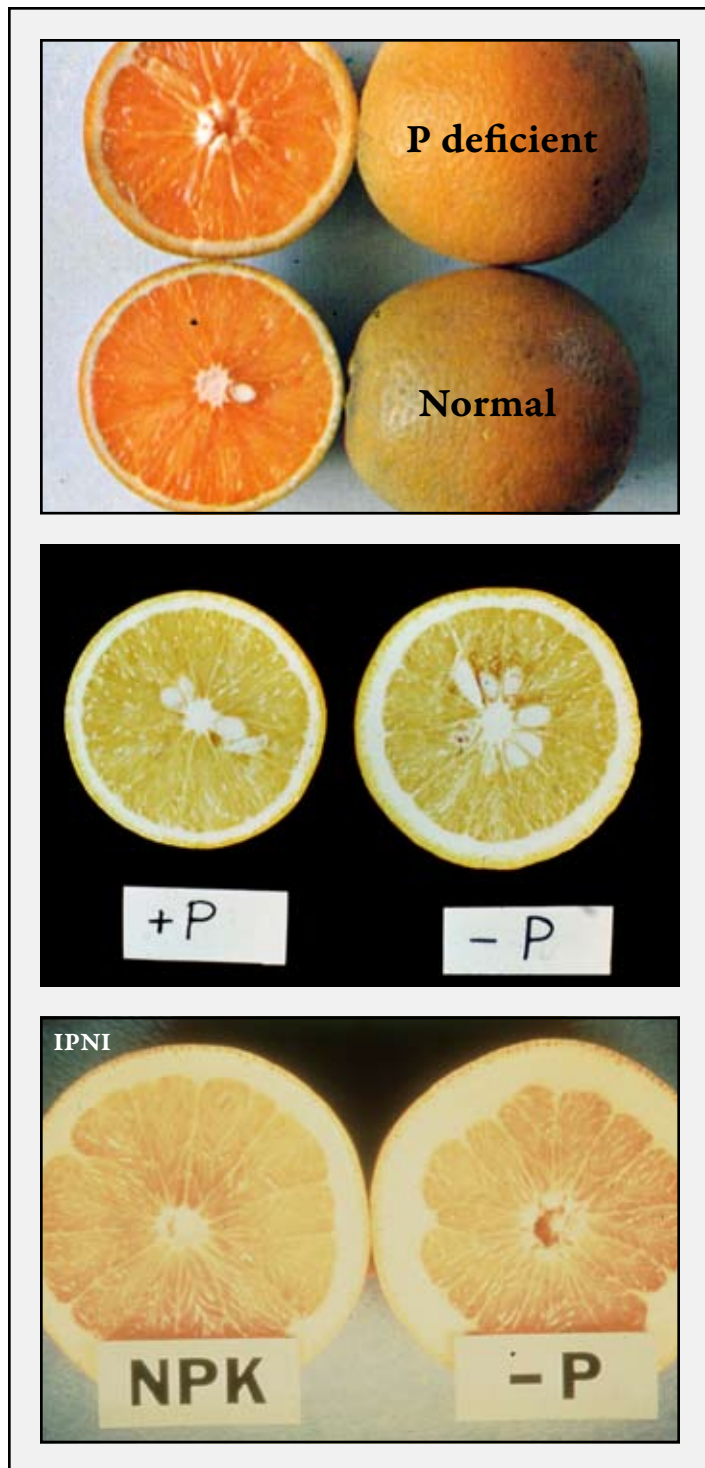
Fig. H2. Phosphorus deficiency. Note the thicker peel and hollow core of P-deficient fruit compared with normal fruit.
