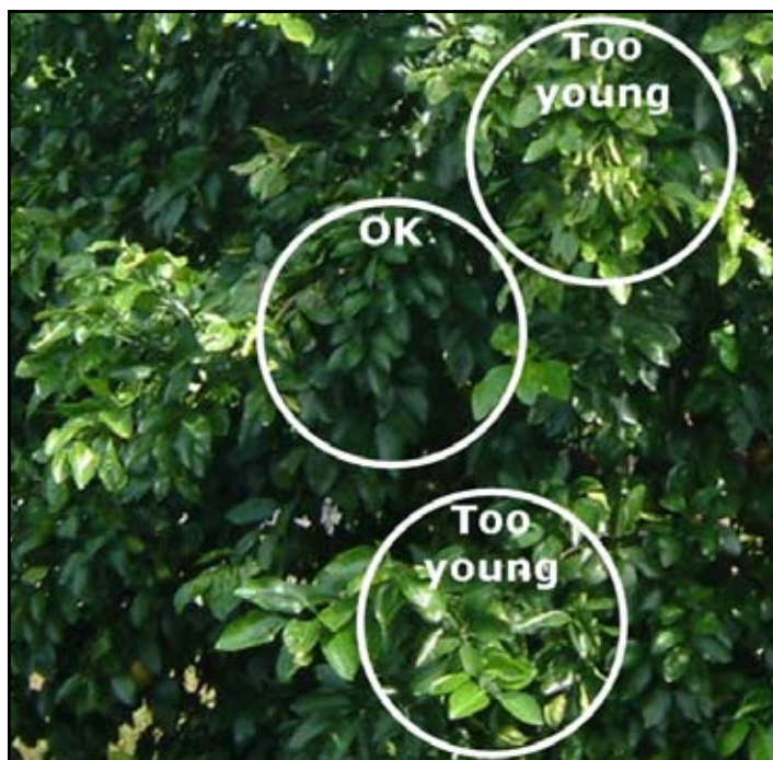
Fig. 4.3. Sample 4 to 6-month-old spring flush leaves from non-fruiting twigs. (Thomas Obreza)
