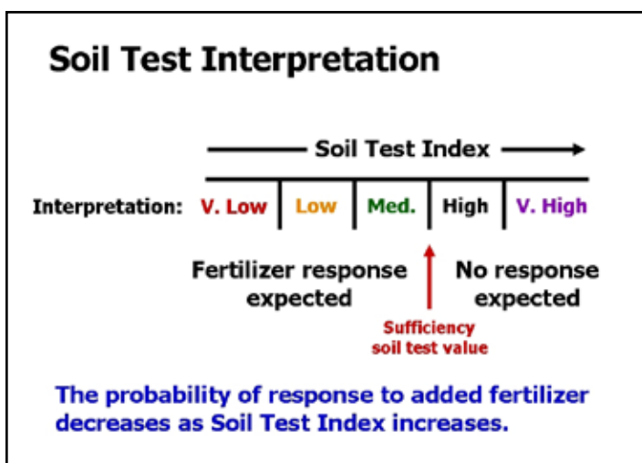
Fig. 4.5. Soil test interpretation categories and their relationship to expected fertilizer response.
